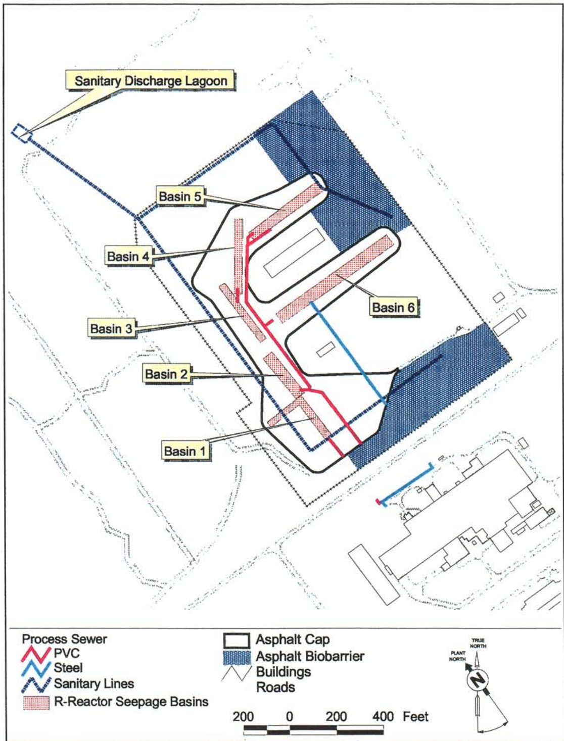
Figure 10. General Layout of the RRSB OU with the Expanded Biobarrier
