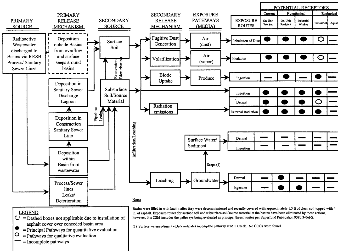
Figure 5. Conceptual Site Model for the RRSB OU
