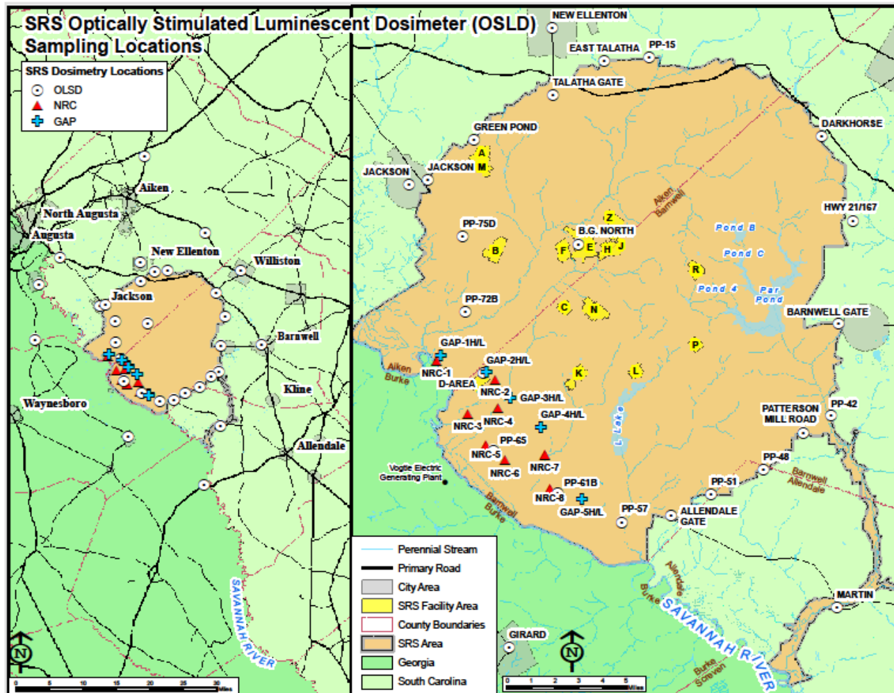
Figure 2 Optically Stimulated Luminescence Dosimeter (OSLD) Sampling Locations
