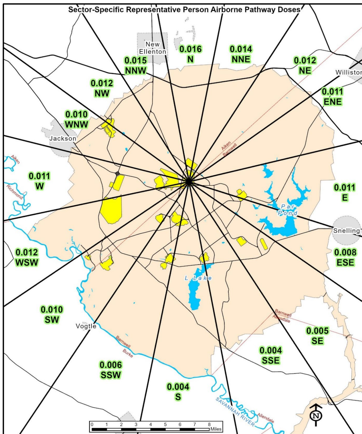
Figure 2-3. Sector-specific Representative Person Site Boundary Doses
