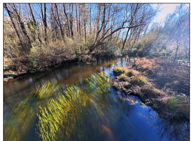
Upper Three Runs is a Southwest-flowing Tributary of the Savannah River.
