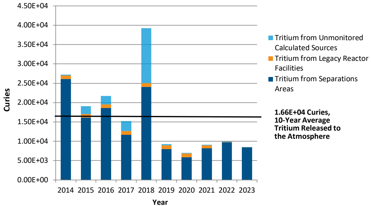
Figure 5-2 10-Year History of SRS Annual Tritium Releases to the Air
